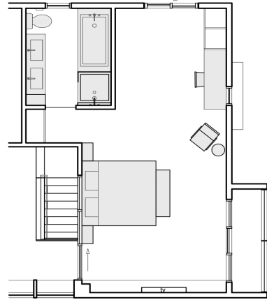
MAIN LEVEL ALT. MASTER BEDROOM PLAN
